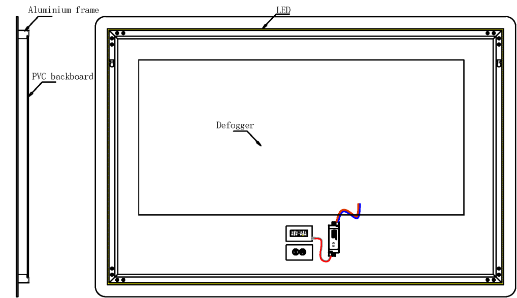
Side View
