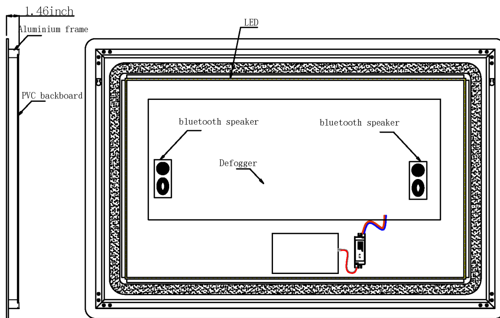
Side View
