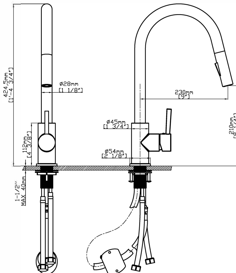
CRITICAL DIMENSIONS
