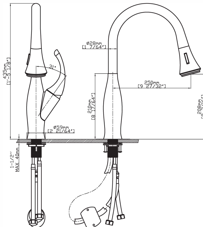
CRITICAL DIMENSIONS
