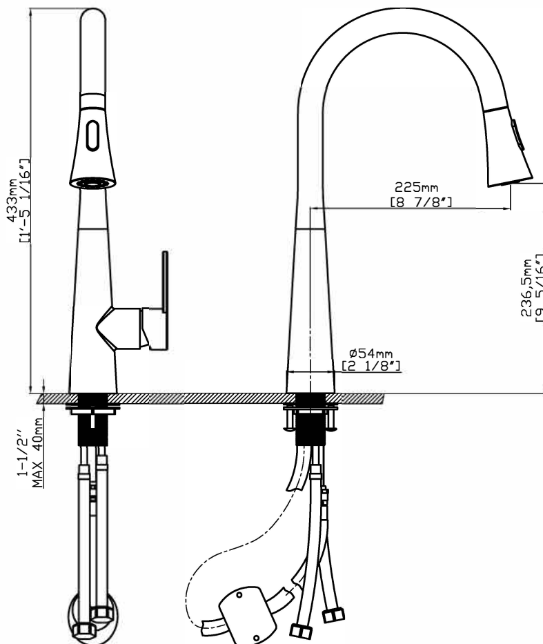
CRITICAL DIMENSIONS
