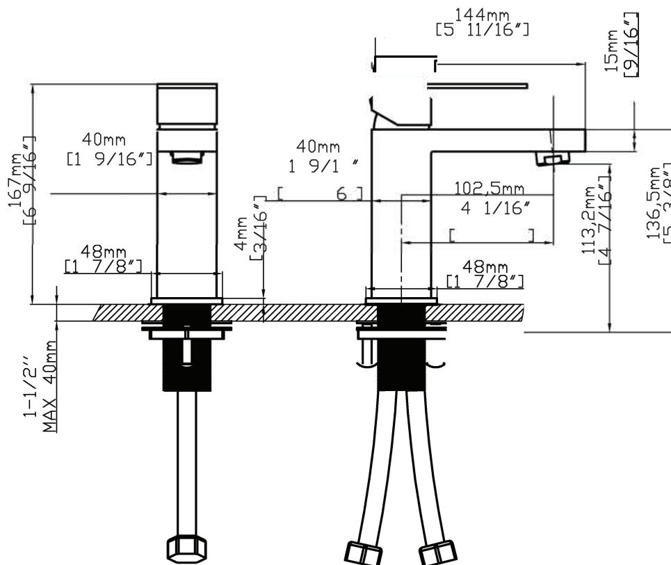
CRITICAL DIMENSIONS
