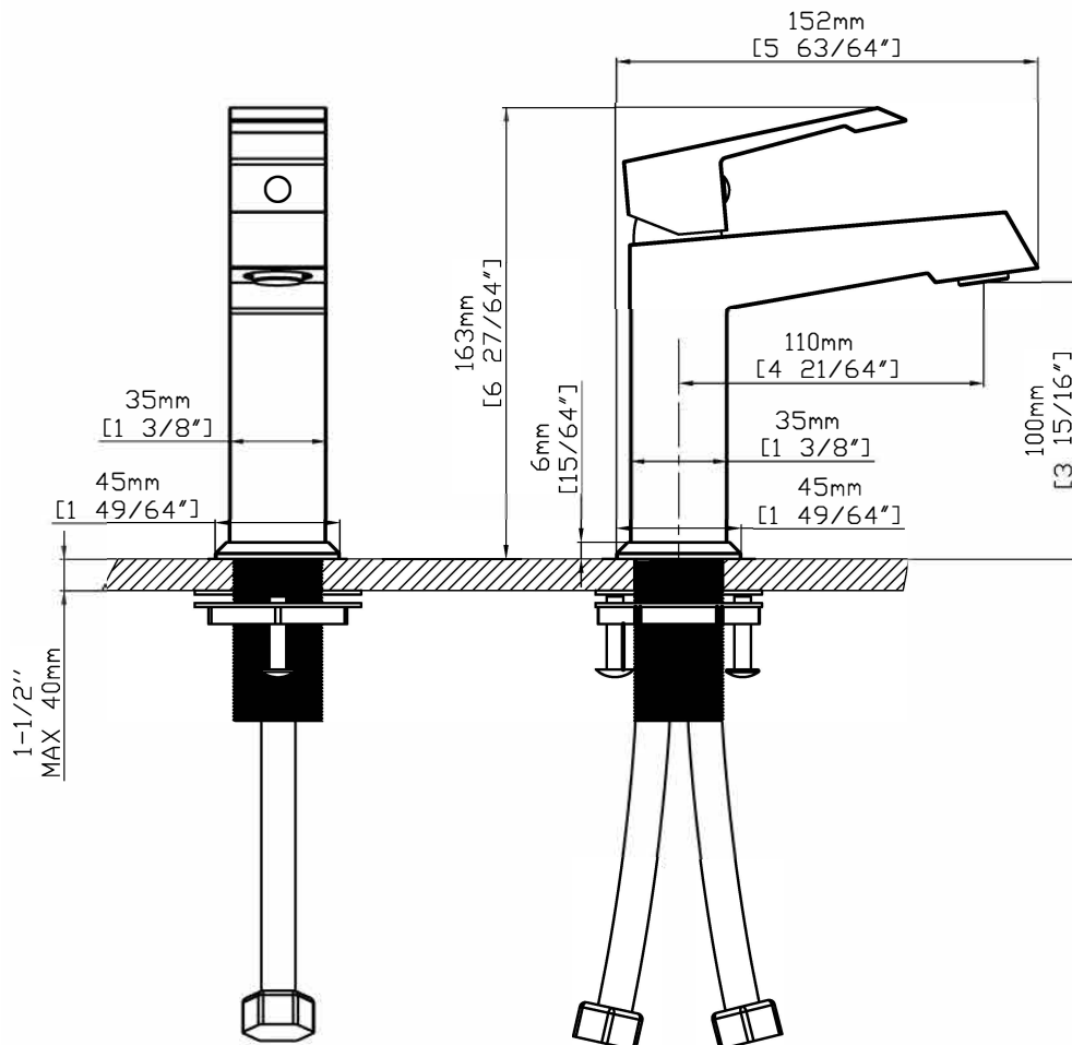
CRITICAL DIMENSIONS
