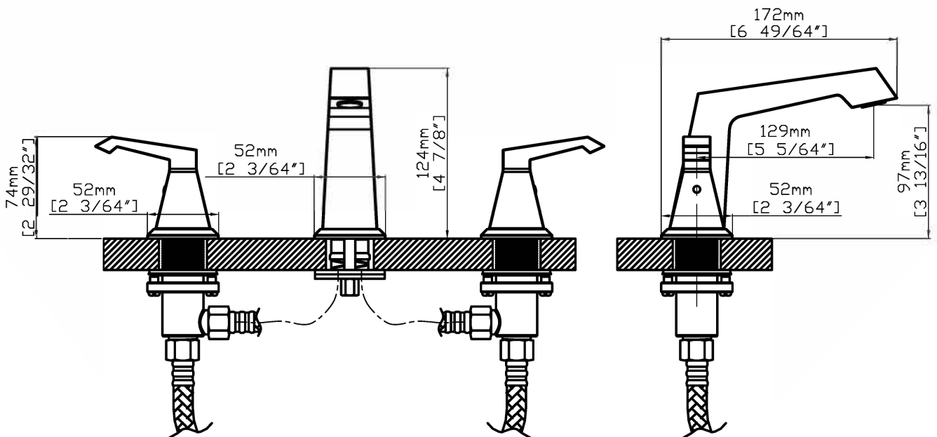
CRITICAL DIMENSIONS
